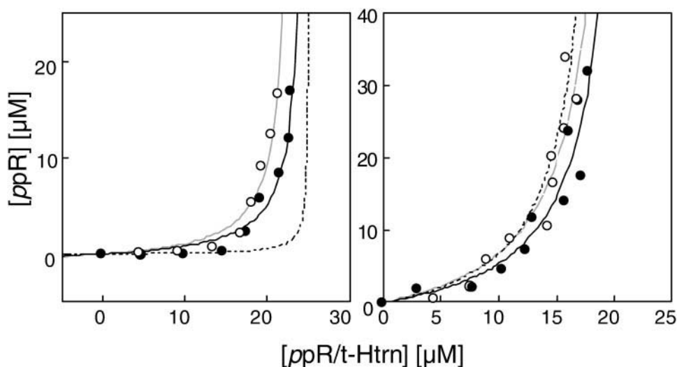
FIGURE 3 Concentrations of the free ppR , [ppR] , plotted against concentrations of the ppR /t-Htr n complex, [ppR/t-Htr_n] during the titration. Details were described by Sudo et al. (2001 and submitted for publication). (A) Plots from the decay rates of the O-like intermediate of the double mutants of Asp-75 and Tyr-199. Open circle, D75N/Y199F; closed circle, D75N/Y199V. The circles are data points; the lines (solid and gray) are regression curves from using nonlinear regression software (Origin, Micalcal, Northampton, MA). The broken line shows the interaction between the O-like intermediate of D75N and t-HtrHis (data from Sudo et al., submitted for publication). The t-Htr concentration was 25 \mu M, and the medium contained 0.1% DM, 400 mM NaCl, 10 mM Tris-Cl at pH 7.0 and 20°C. (B) Plots from the decay rates of the M-like intermediate of Tyr-199 mutants. Open circle, Y199F; closed circle, Y199V. The circles are the data points; the lines (solid and gray) are regression curves. The broken line shows the interaction between the M-intermediate of the wild-type and t-Htr (data from Sudo et al., 2001). The t-Htr concentration was 25 \mu M, and the medium composition and temperature were the same as for (A). The curves of (A) are steeper than those of (B) because Asp-75 mutants have a greater affinity (smaller K_D ) for the transducer. Table 1 lists estimated K_D and n .
