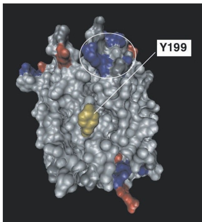
FIGURE 2 X-ray crystallographic structure of ppR (Royant et al., 2001; 1H68 of PDB code). The surface patch (circle) on the cytoplasmic side of ppR is a putative binding site suggested by Royant et al. (2001). Tyr-199 on face I is another putative binding site of ppR (Luecke et al., 2001) and is in the middle of the transmembrane helix of G.
