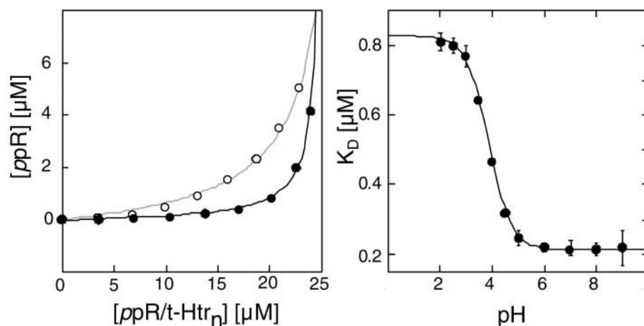
FIGURE 5 K_D values of the D75N/t-Htr complex at varying pH. (A) The titration of t-Htr (25 \mu M) with ppR at pH 2 (open circles) and pH 6 (closed circles). Data were fitted by the same method as described for Fig. 2. (B) K_D values estimated are plotted against pH. The solid curve is a fitted curve by using the Henderson-Hasselbach equation with pK_a of 3.86 \pm 0.02 . The experimental conditions were the same as for Fig. 3.
